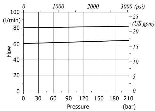
VPR/3/ET/RL/VMP 34 pressure compensation diagram (E→C)
